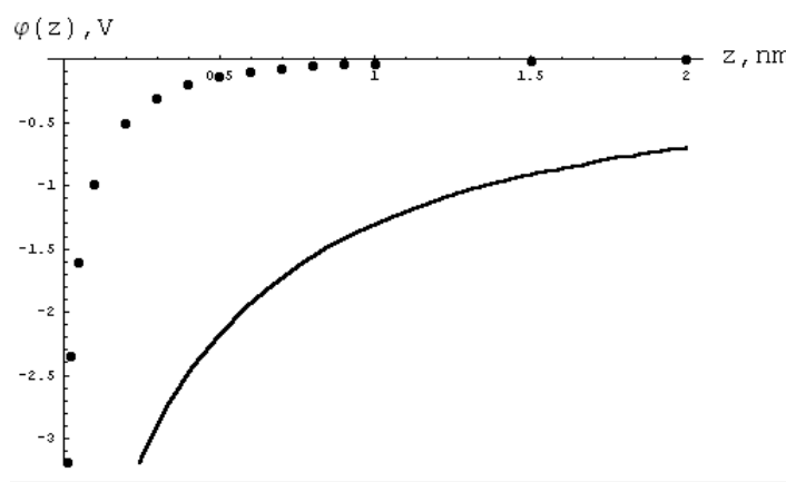
Figure 1: The screened potential \varphi(z) according to (2.14) for the (5, 5) nanotube (plotted point by point) in comparison with the unscreened averaged Coulomb potential (solid line)
